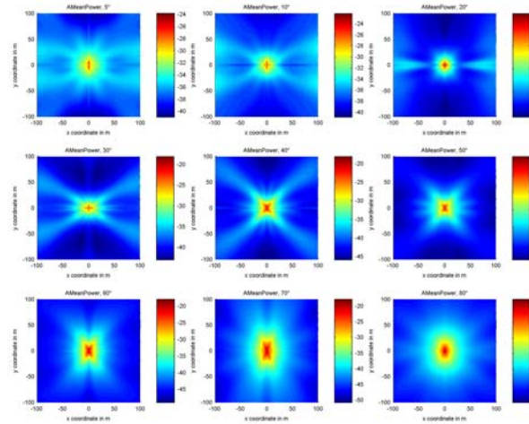
Figure 28: Mean power of reflections in dependency of their position – Suburban case in dependency of the elevation
